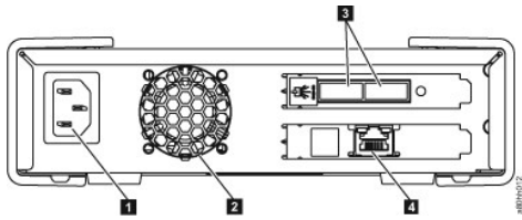
Figure 6. Rear Panel of External SAS Tape Drive
